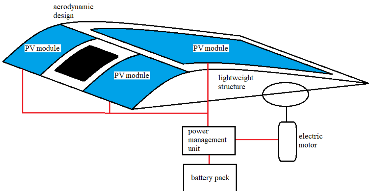
Figure 3 Solar car diagram and components.
