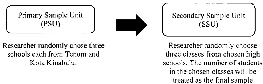
Figure 1: Stens in Two-Stage Cluster Sampling.
